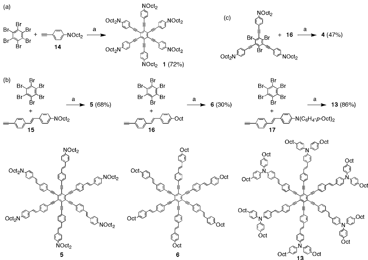
Scheme 1. Synthesis of 1 , 4 , 5 , 6 , and 13 . Reagents and conditions: (a) arylacetylenes (9–12 equiv), PdCl 2 (PPh 3 ) 2 (7–10 mol %), CuI (14–20 mol %), PPh 3 (14–20 mol %), Et 3 N, reflux.
